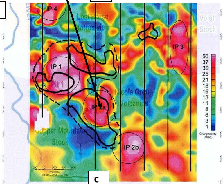
Plan View Titan 24 Chargeability Anomaly
