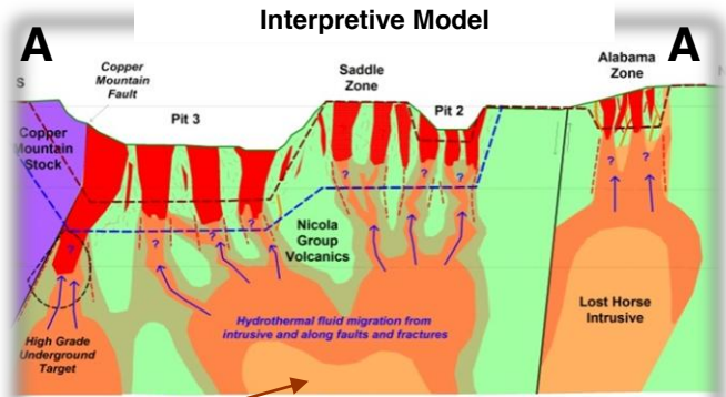
Schematic cross-section model of mineralization in Copper Mountain
