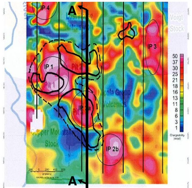
Plan View of Chargeability Model
